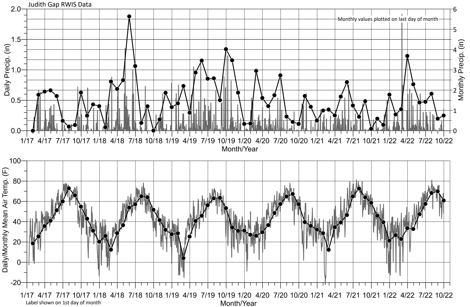
Figure 10. Judith Gap RWIS Time History Plot
